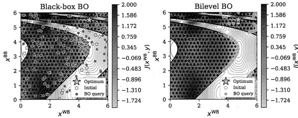
Figure 3: Small-Feasible-Region 2: same layout as Figure 2. Here the black-box function is nonlinear ( y = \frac{x^{\text{BB}} - 5.5}{2} \exp(x^{\text{BB}}/2) ), distorting the relationship between x^{\text{BB}} and the feasible set. Bilevel BO still concentrates near the optimum because the GP surrogate learns the scalar mapping x^{\text{BB}} \mapsto J(x^{\text{WB}*}) in one dimension.
