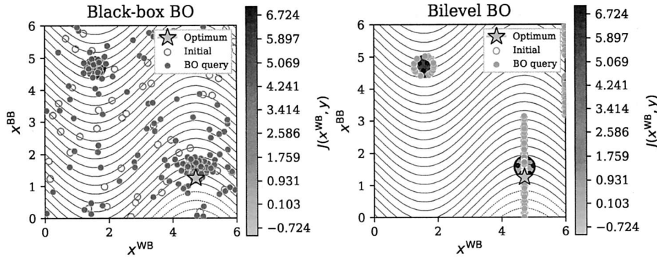
Figure 2: Small-Feasible-Region 1: search behavior of black-box BO (left) and bilevel BO (right) after 50 initial samples + 200 BO iterations. Background: objective J(x^{\text{WB}}, y) (yellow = low); white regions are infeasible; hatching marks feasible islands; \star marks the global optimum. Black-box BO scatters queries across the full (x^{\text{WB}}, x^{\text{BB}}) space. Bilevel BO concentrates concentrates along the x^{\text{BB}} axis—each query selects an x^{\text{BB}} value, and the inner NLP finds the best feasible x^{\text{WB}} .
